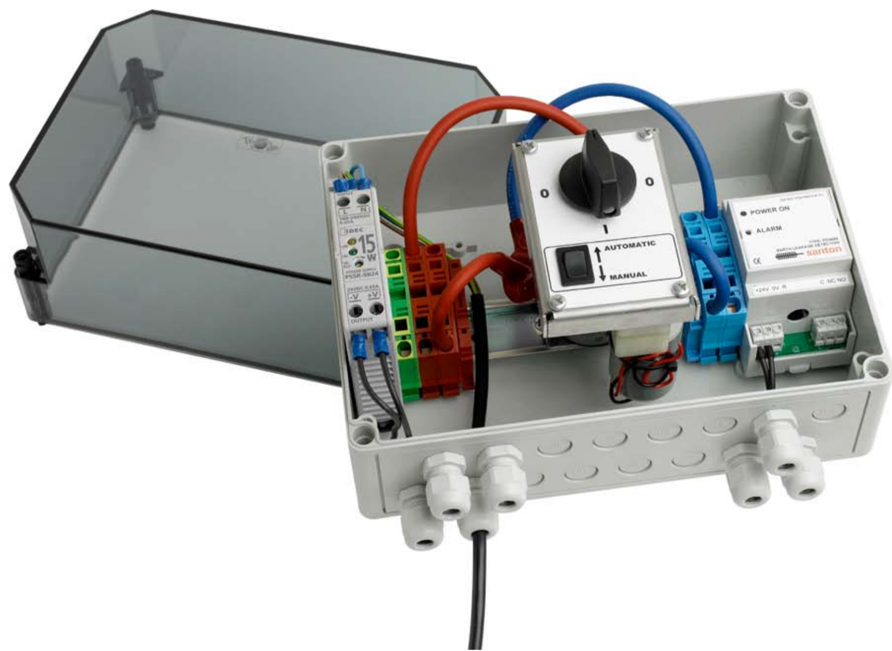
Santon junction box with a 25 A/1000VDC/2P motor driven switch and earth fault detection It allows to isolate the inverter from the PV field and gathers four strings (configurable). Detects earth faults through an electronic relay that operates the switch in alarm conditions
