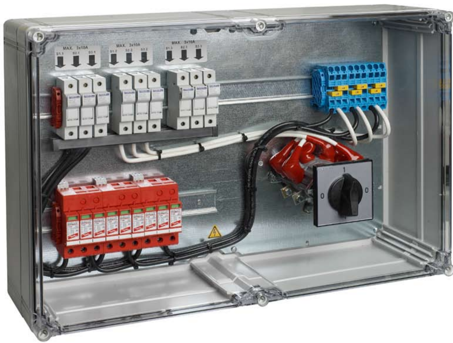
Santon junction box 40A/900VDC/ 6P With fuses and overvoltage protection type II Suitable for a multistring inverter with three inputs
