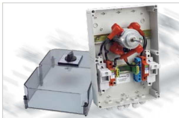
40A 900 V DC with fuse holders
