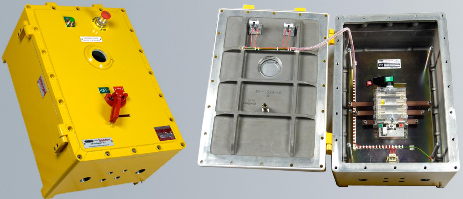
160A Isolator for EExd / ATEX hazardous areas
